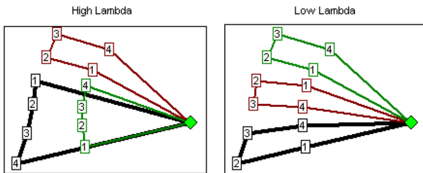
Figure 26-Lambda
